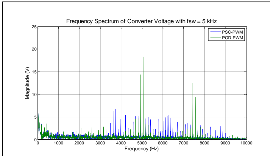
Figure 4.40 Frequency Spectrum for PSC-PWM and POD-PWM at f_{sw}=5\text{kHz}
