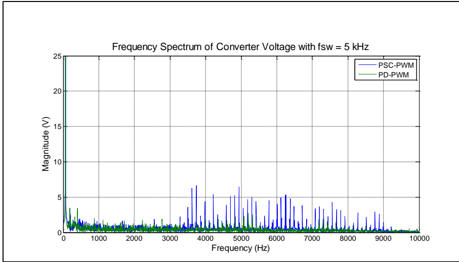
Figure 4.39 Frequency Spectrum for PSC-PWM and PD-PWM at f_{sw} = 5 \text{ kHz}
