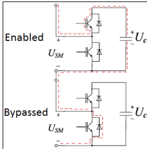
Figure 1.6 Converter Conduction Path, Negative Current
