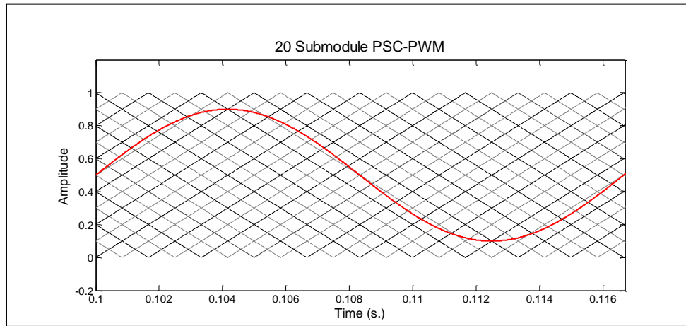
Figure 2.3 PSC-PWM
