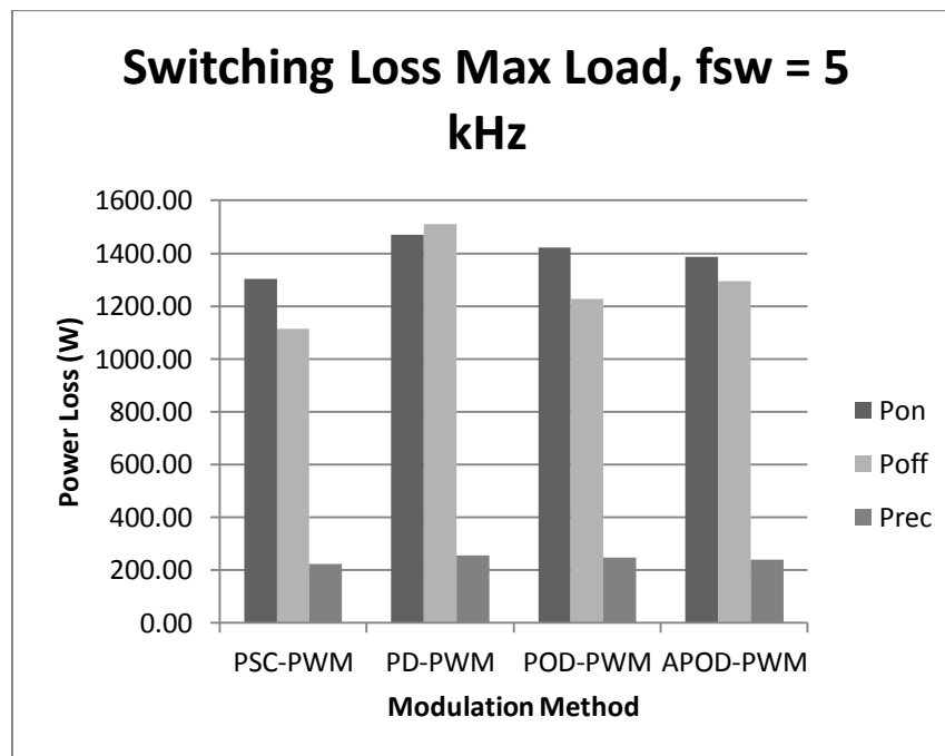
Figure 4.24 Per SM Switching Loss using Conventional Voltage Balancing, 5 kHz
